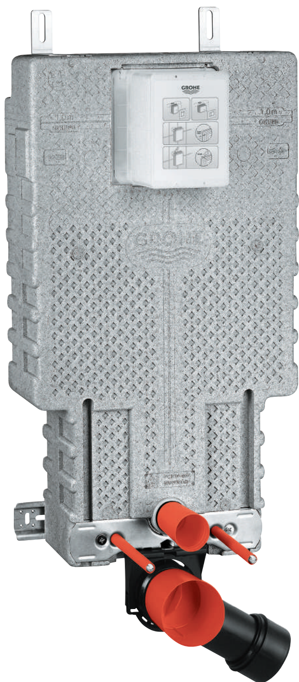
38 643 001 Uniset for WC with flushing cistern 6 - 9 ltr. dual flush/start & stop/single flush, water supply from the left, right, rear or top for walling in
